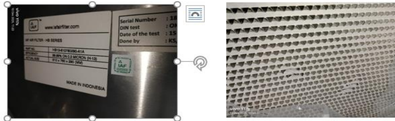
HEPA Filter HB Series H14 double header
